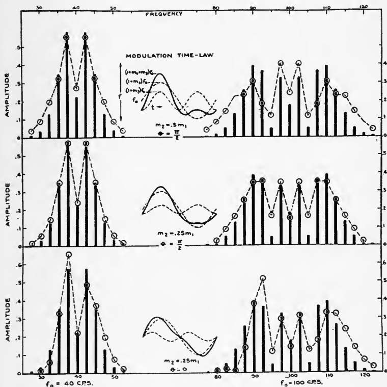
FIG. 6. Effect of departures from sinusoidal modulation. Vertical bars represent spectral distribution of sinusoidal modulation of \approx 12.5\% at 2.5 cps. Circles represent spectral distribution for modulation illustrated and defined by
